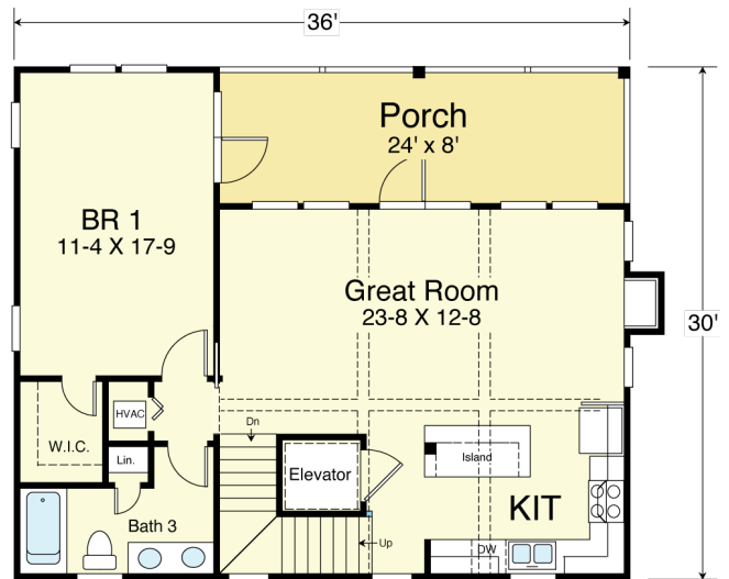
SECOND FLOOR PLAN 888.0 S.F. 9'-0" Flat Ceiling Heights
