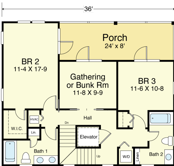
FIRST FLOOR PLAN 888.0 S.F. 8'-0" Ceiling Heights
