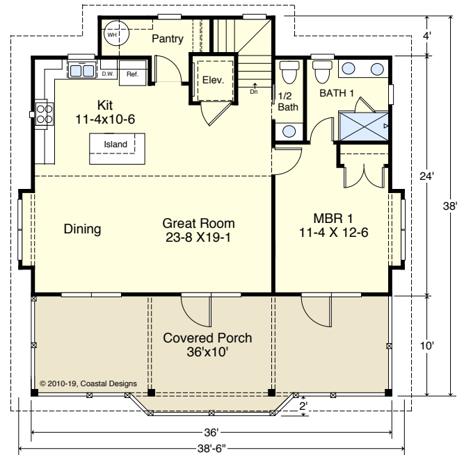
2nd FLOOR 954.7 SF 9' ceiling heights
