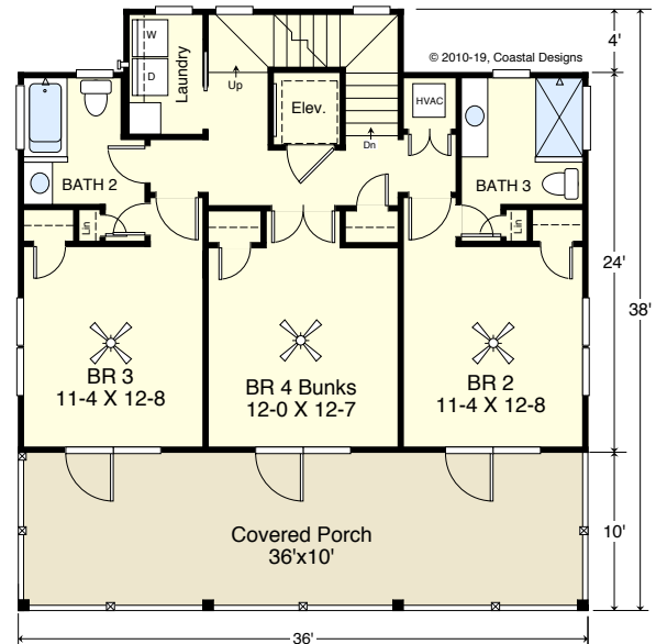
1st FLOOR 934.7 SF 8' ceiling heights
