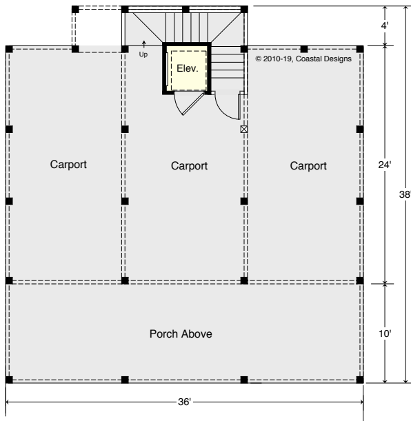
GROUND FLOOR 25.8 SF (Elevator) 8' ceiling heights
