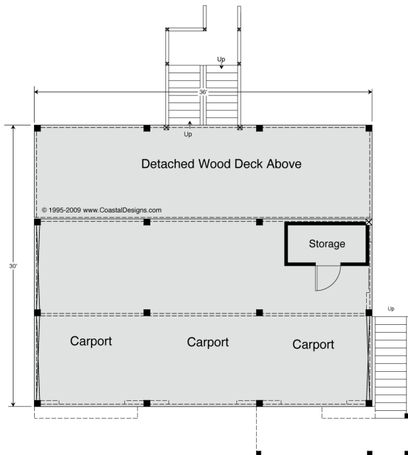
GROUND FLOOR PLAN 8' Ceilings
