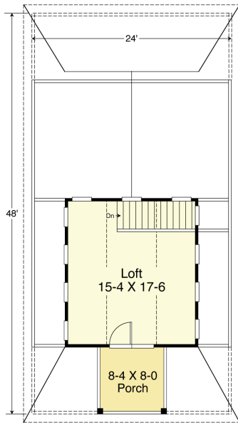
THIRD FLOOR PLAN (LOFT) 283.5 s.f. 8' Sloping Ceilings
