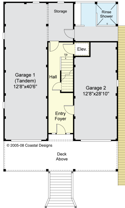
GROUND FLOOR PLAN 8' Ceilings
