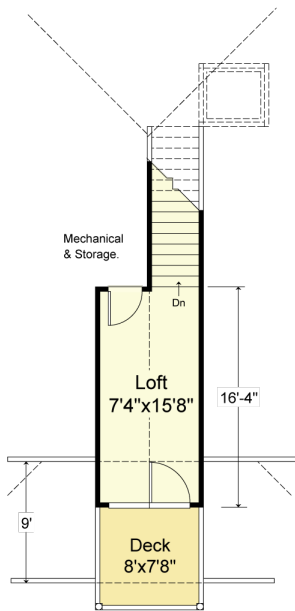
THIRD FLOOR PLAN (LOFT) 8' Ceilings
