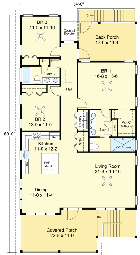
FIRST FLOOR PLAN 9' Flat Ceilings
