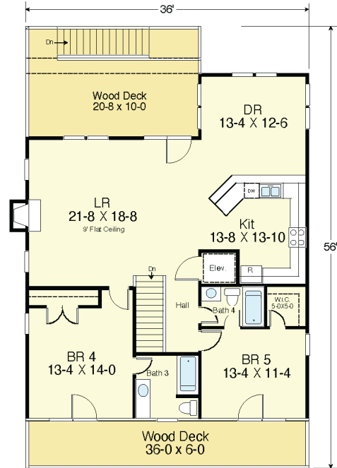
SECOND FLOOR PLAN 9' Flat Ceilings 1,408 S.F.
