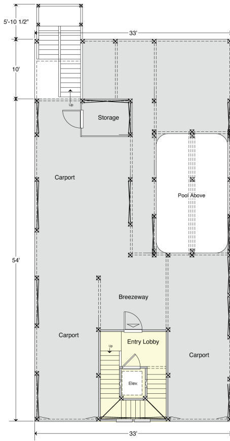
GROUND FLOOR PLAN 178.9 S.F. (Unheated)
