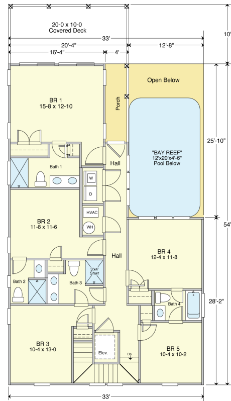
SECOND FLOOR PLAN 33' x 54' (box) = 1,402.1 S.F. 8' Ceilings
