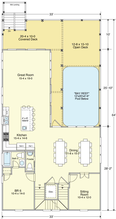
FIRST FLOOR PLAN 33' x 54' (box) = 1,351.2 S.F. 9' Ceilings
