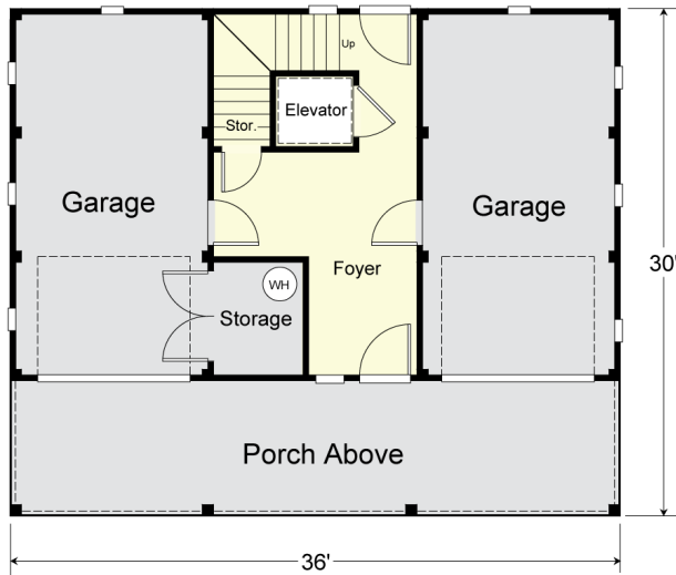
GROUND FLOOR PLAN 8'-0" Ceilings
