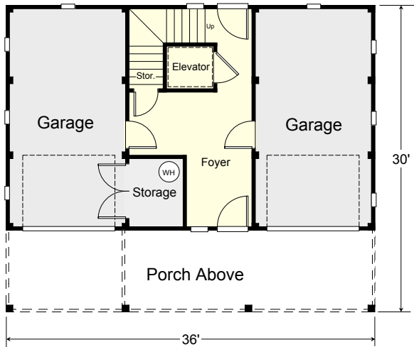
GROUND FLOOR 190.0 SF 8' ceiling heights
