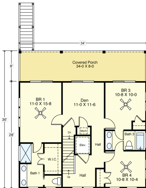
FIRST FLOOR PLAN 952.0 S.F. 8'-1 1/2" Ceilings
