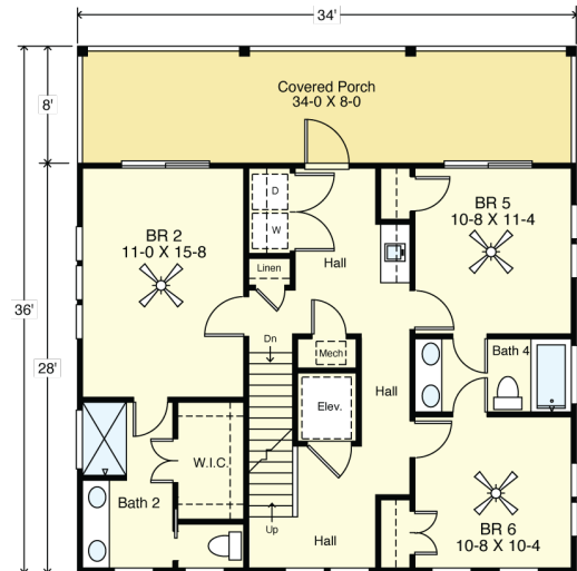
SECOND FLOOR PLAN 952.0 S.F. 8'-1 1/2" Ceilings
