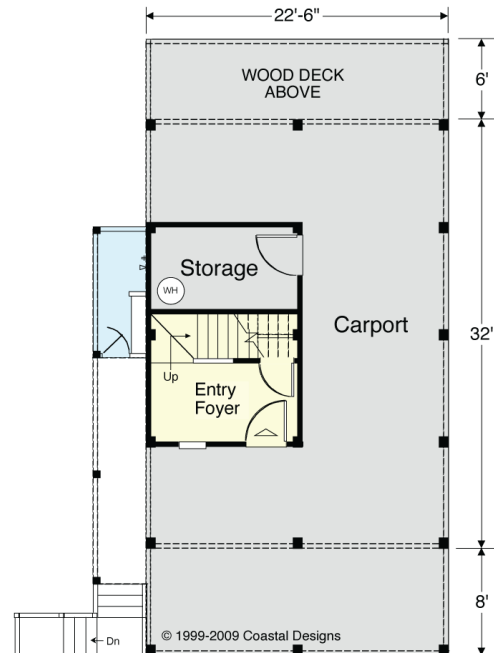
GROUND FLOOR PLAN (OPTIONAL) Optional Bad Weather Entry
