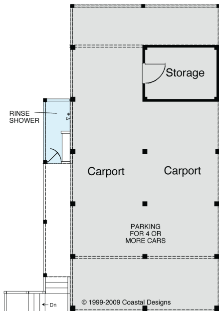
GROUND FLOOR PLAN Open Carports
