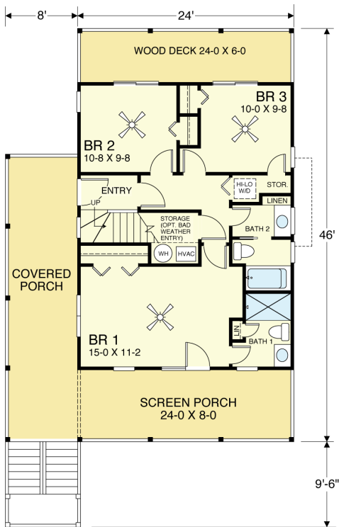
FIRST FLOOR PLAN 768.0 SF 8'-0" Ceilings
