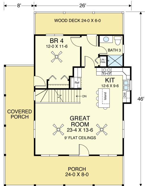
SECOND FLOOR PLAN 768.0 S.F. 9'-0" Flat Ceilings (Vaulted Ceiling Optional in Great Room)
