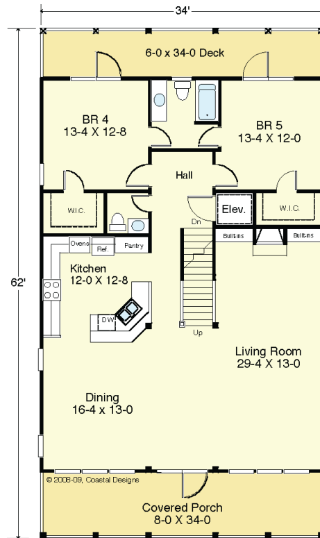
SECOND FLOOR PLAN Living Area 1,632.0 S.F. Deck Area 272.0 S.F. 9'-0" Ceilings
