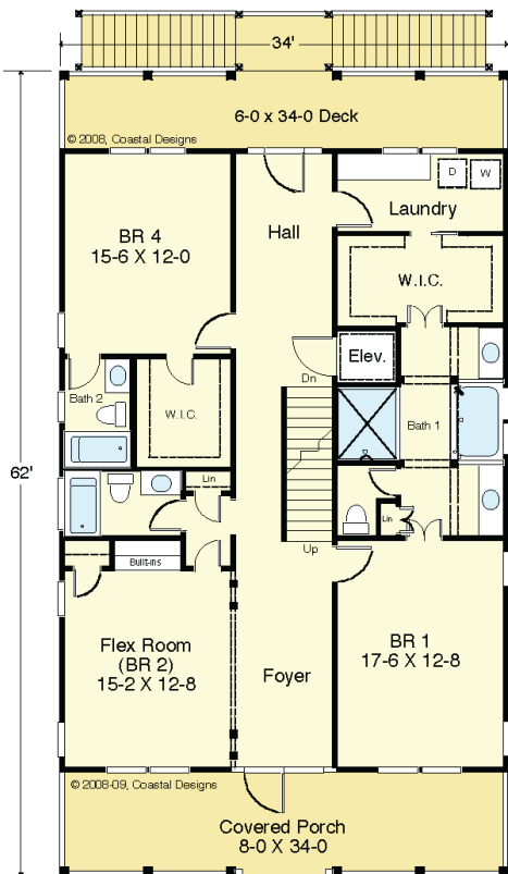
FIRST FLOOR PLAN Living Area 1,632.0 S.F. 8'-0" Ceilings
