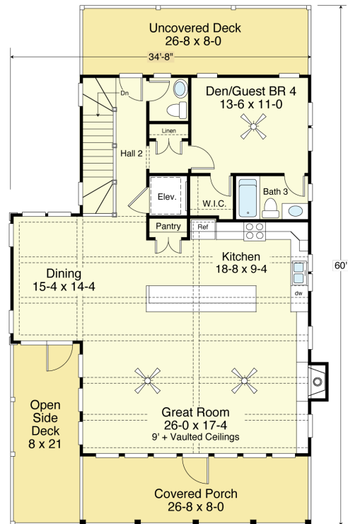
SECOND FLOOR PLAN 1,308.0 S.F. 9'-0" Ceiling Heights
