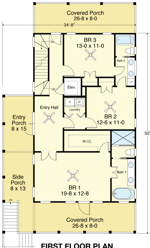
FIRST FLOOR PLAN 1,173.3 S.F. 8'-0" Ceiling Heights and 4" Exterior Walls
