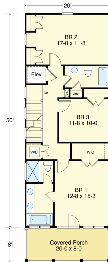
SECOND FLOOR PLAN 1,000.0 S.F. 9'-0" Ceiling Height
