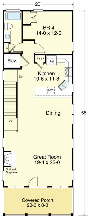
FIRST FLOOR PLAN 1,000.0 S.F. 9'-0" Ceiling Height
