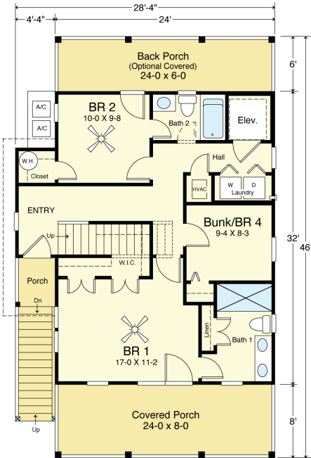
FIRST FLOOR PLAN 820.0 S.F.
