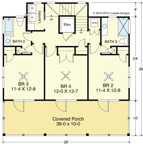
ALTERNATE FIRST FLOOR PLAN
