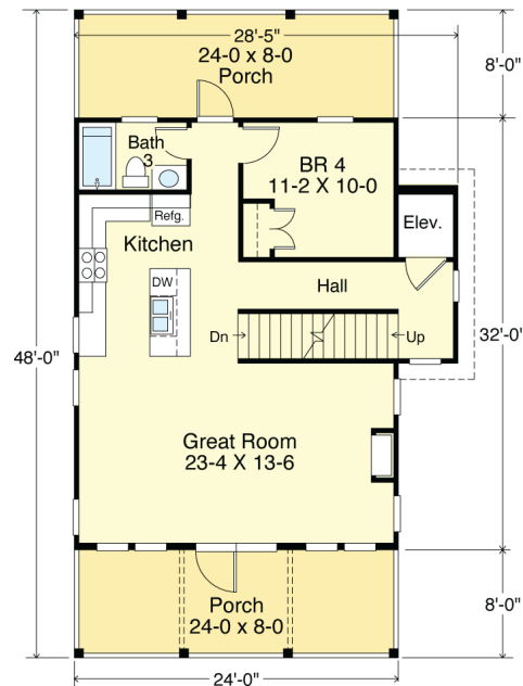
SECOND FLOOR PLAN 827.6 S.F. 9'-0" Ceiling Height
