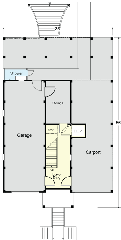
GROUND FLOOR PLAN 9' Ceilings
