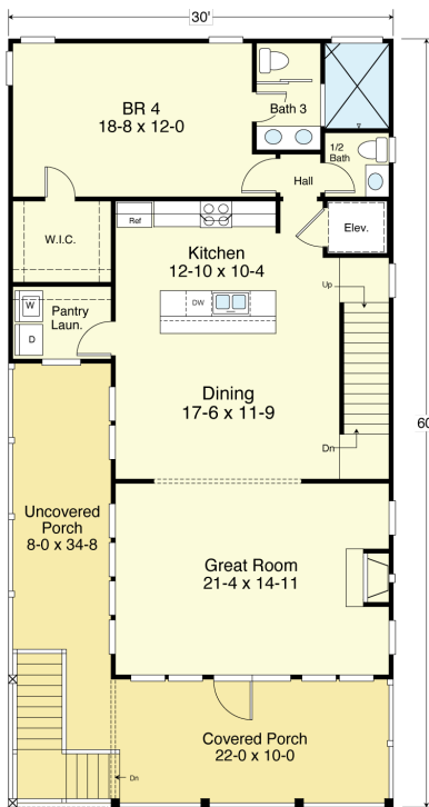
FIRST FLOOR PLAN 1,302.7 S.F. 9'-0" Ceiling Height
