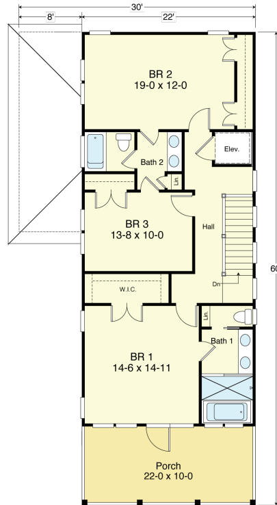
SECOND FLOOR PLAN 1,100.0 S.F. 9'-0" Ceiling Height
