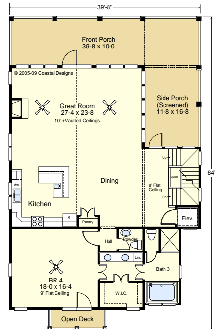
2nd Floor Plan Living Area = 1,714.2 s.f. 9' & 10' + Vaulted Ceilings
