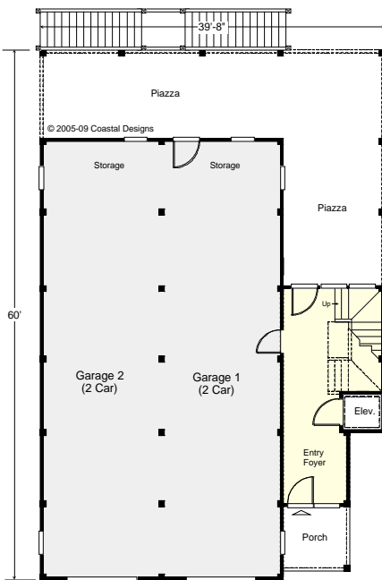
Ground Floor Plan Entry Area = 258.3 s.f. Garage = 1,400.0 s.f. 8' Flat Ceiling Height
