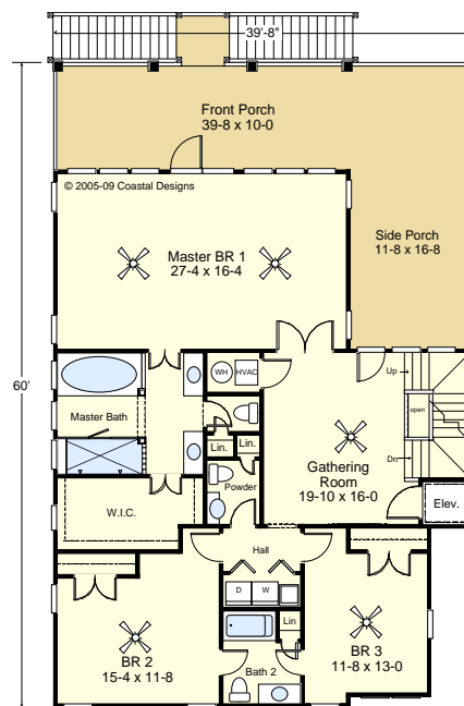
1st Floor Plan Living Area = 1,714.5 s.f. 9' Flat Ceilings
