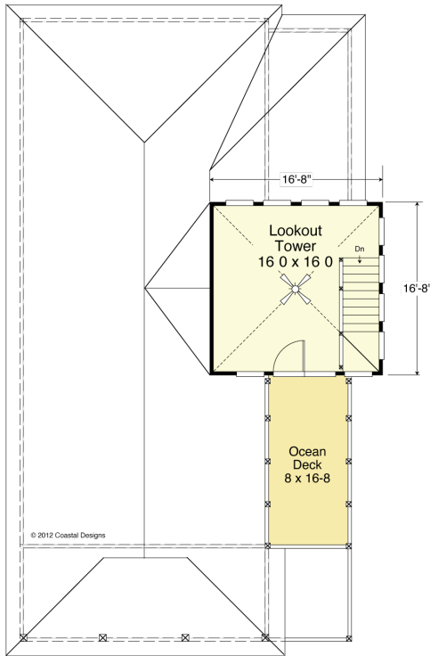
THIRD FLOOR (LOFT) PLAN
