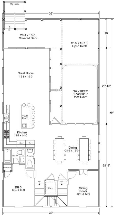
FIRST FLOOR PLAN 33' x 54' (box) = 1,351.4 S.F. 9' Ceilings
