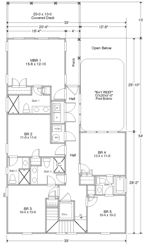
SECOND FLOOR PLAN 33' x 54' (box) = 1,402.1 S.F. 8' Ceilings
